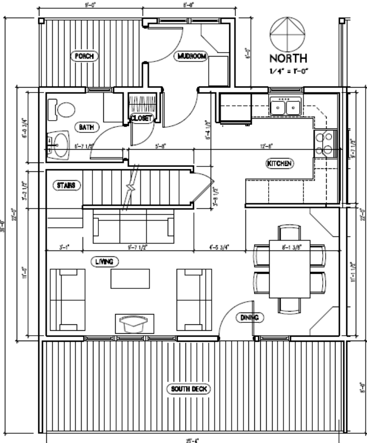
1st Floor
